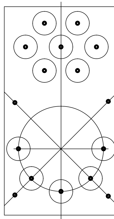
Drilling Template for Lid
