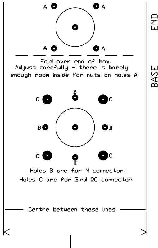
Drilling Template for End and Base of Box
